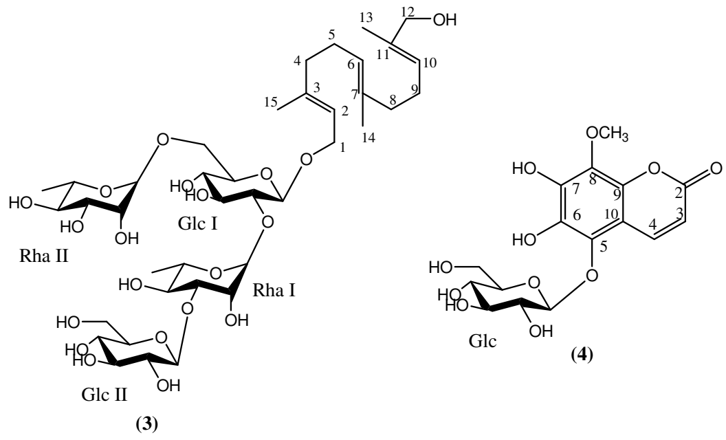
Fig. 1. Structures of isolated compounds 1–5
