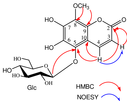
Fig. 2d. Key HMBC and NOESY correlations observed for Compound 4
