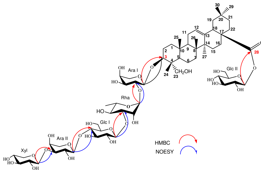
Fig. 2a. Key HMBC and NOESY correlations observed for Compound 1
