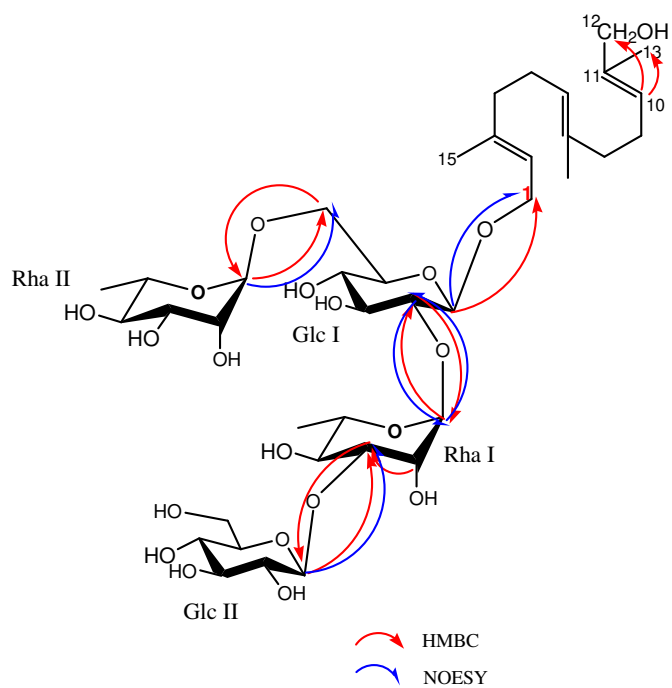
Fig. 2c. Key HMBC and NOESY correlations observed for Compound 3
