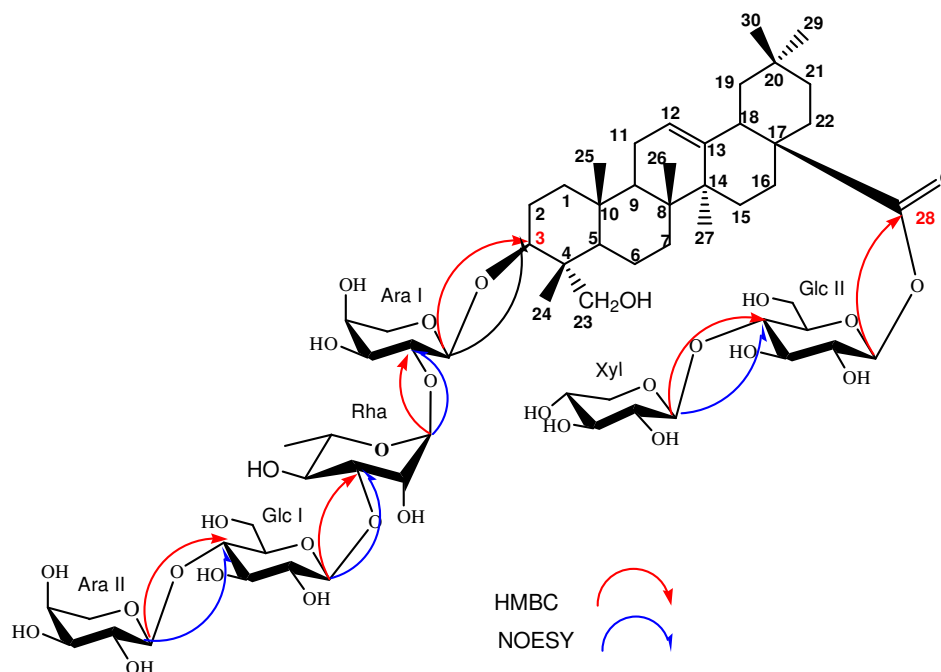
Fig. 2b. Key HMBC and NOESY correlations observed for Compound 2
