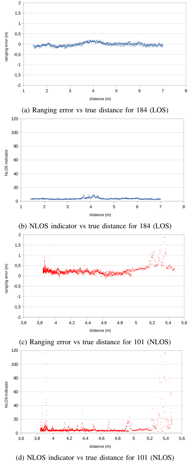
Fig. 13: Representation of the NLOS indicator using UWB-TWR
