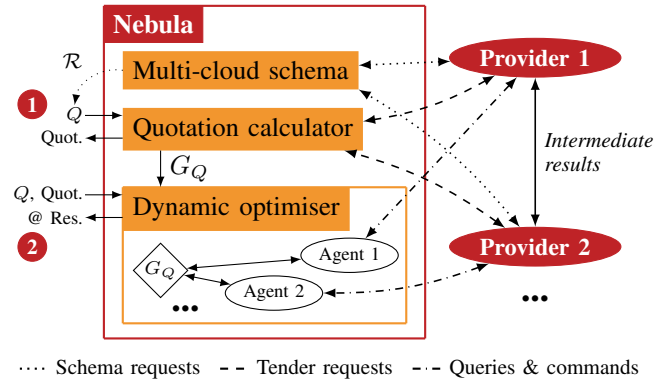
Figure 1. Overall design of the Nebula system.
