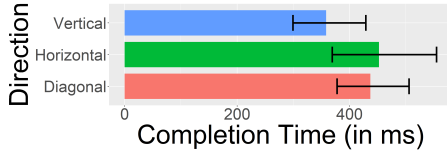
Figure 7: Precise Head Point completion time according to direction (in ms) with 95% CI
