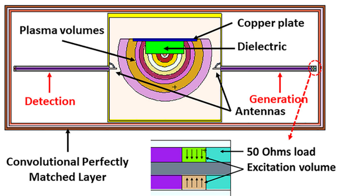
FIG. 11. Cavity modeling with plasma shells.
