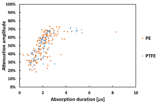
FIG. 8. Microwave transmission characteristics.
