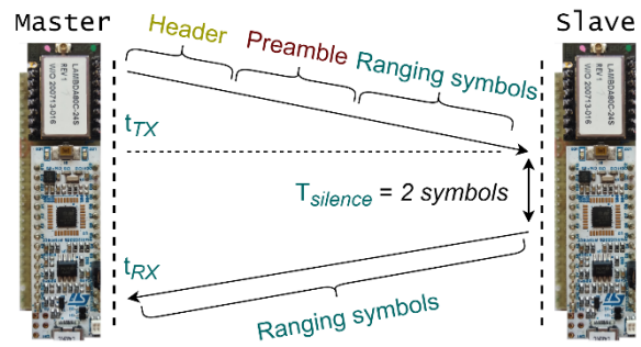
Fig. 3. Ranging protocol between 2 LoRa-2.4GHz ranging nodes
