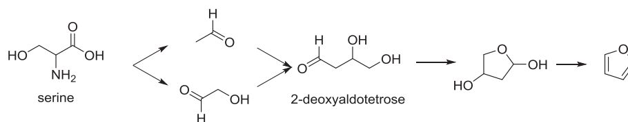
Figure 3: Suggested formation pathway of furan from serine (adapted from Perez Locas and Yaylayan, 2004; Limacher et al., 2008)
