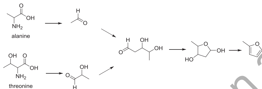
Figure 6: Suggested formation pathway of 2-methylfuran (adapted from Märk et al., 2006)
