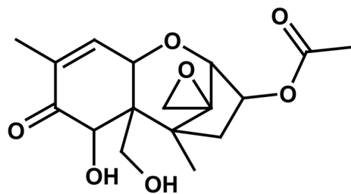
3-acetyldeoxynivalenol (3-ADON)
