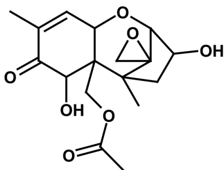
15-acetyldeoxynivalenol (15-ADON)
