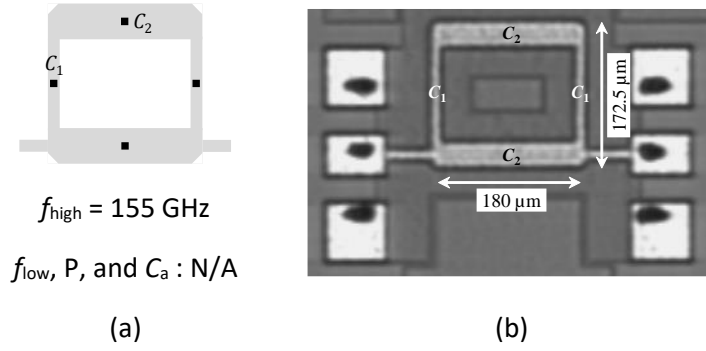
Fig. 12. (a) Layout representation and (b) photography of the 155 GHz ring filter.
