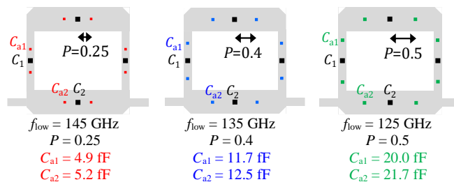
Fig. 16. Layout representations of the ring resonators having the same 17-GHz natural bandwidth.
