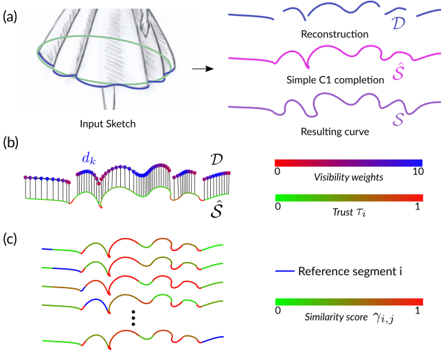
Figure 5: Completing occluded portions of the folded hemline. a) The input curve \mathcal{D} is incomplete. A first initial continuous guess curve is generated \hat{S} to fill the missing parts, and is further deformed into the final approximating folded curve S . b) The projection of samples of \mathcal{D} onto \hat{S} are used to measure a trust score \tau_i and a per-sample visibility weight. c) Bézier segments are compared together using a geometrical similarity score \gamma_{i,j} .
