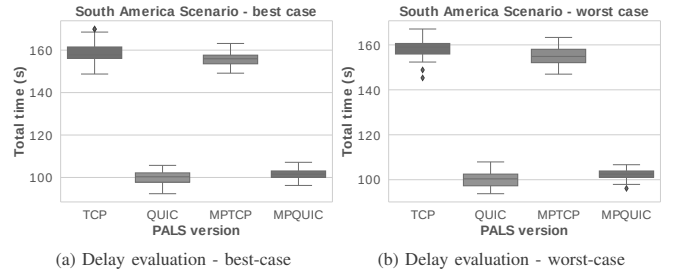
Fig. 10: South America evaluations
