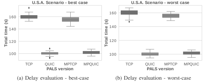
Fig. 9: United States of America evaluations
