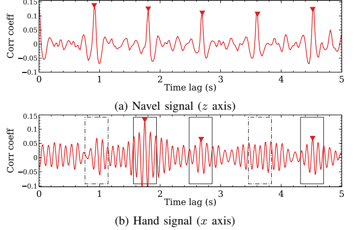
Fig. 4: Cross-correlation of the signal with a 1-s-long slice centered at the maximum amplitude. Ground truth heart rate: 65 bpm ( \sim 5.4 pulses in 5 s window)
