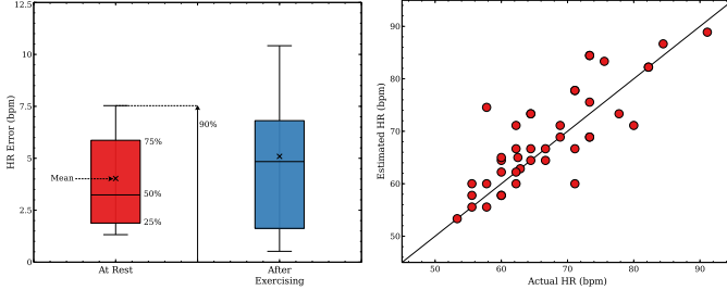
(a) Performance at rest and after (b) Performance at different heart rates
