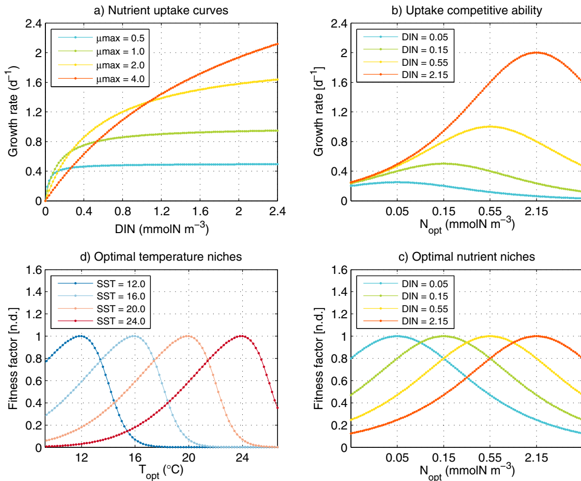
Fig. 2. Optimal niches of nutrient concentration ( N_{\text{opt}} ; \text{mmol N m}^{-3} ) from gleaners to opportunists as a function of dissolved inorganic nitrogen DIN, and optimal niches of temperature ( T_{\text{opt}} ; ^{\circ}\text{C} ) from colder to warmer preference as a function of sea surface temperature SST for the highest functional diversity phytoplankton community. (a) The resource uptake [ \text{d}^{-1} ] curves of the four uptake strategies result from a trade-off between uptake affinity and maximum growth rate ( \theta \cdot \mu_{\max} = \text{constant} ): slow-growing gleaners are superior competitors at low nutrient concentration because they have a higher nutrient affinity, while fast-growing opportunists are superior competitors at high nutrient concentration because they have a higher maximum growth rate. Thus each \mu_{\max} corresponds to a different N_{\text{opt}} . (b) The competitive fitness \text{d}^{-1} of the uptake strategies depends on the nutrient concentration (e.g. when \text{DIN} = 0.05 \text{ mmol N m}^{-3} the fastest uptake corresponds to nutrient gleaners; when \text{DIN} = 2.15 \text{ mmol N m}^{-3} the fastest uptake corresponds to nutrient opportunists). (c) The fitness factor [n.d.] (i.e. competitive fitness normalized by its maximum value) reveals more clearly the nutrient niches as a function of the resource uptake strategy. (d) The fitness factor [n.d.] of the thermal niches depends on the ocean temperature. A total of four optimal uptake strategies (c) and four optimal temperature preferences (d) lead to a combination of 4 \times 4 = 16 ecological niches ( N_{\text{opt}}, T_{\text{opt}} ), each of them filled by one of the 16 phytoplankton species present in the community.
