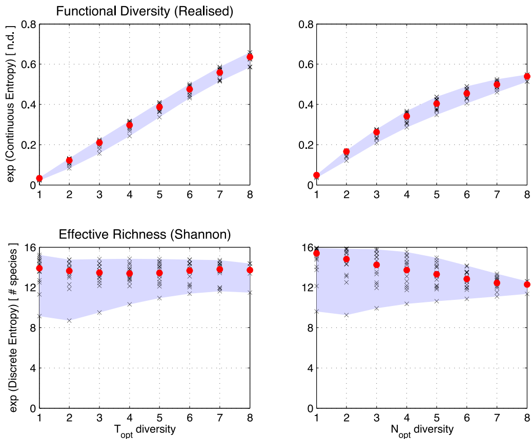
Fig. 6. Functional diversity (exponential of the differential entropy of the continuous probability density function pdf( N_{opt} , T_{opt} ), normalized by its maximum value; n.d.) and effective species richness (exponential of the Shannon diversity index; # species) for the annually-averaged phytoplankton community as a function of the diversity in thermal preferences (left panels) and the diversity in nutrient uptake strategies (right panels). This figure gives the distribution of values resulting from the 1024 simulations that were performed. The red dots correspond to the median value of the distribution. The gray shaded area spans from the minimum to the maximum value of the distribution. Increasing the diversity of thermal and/or uptake strategies preferences of the phytoplankton community leads to a strong increase in the median, minimum and maximum value of the functional diversity while the effective richness remains constant and close its maximum value. (For interpretation of the references to colour in this figure legend, the reader is referred to the web version of this article.)
