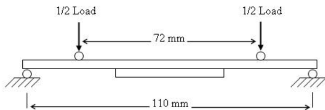
Fig. 2: Specimen geometry and configuration, unit: mm and Four-point bending test principle
