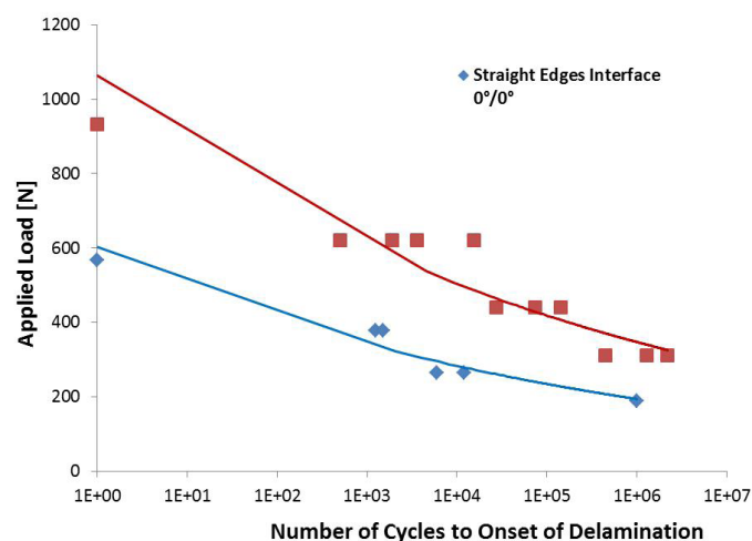
Fig. 6: Comparison to onset delamination between straight and tapered configuration
