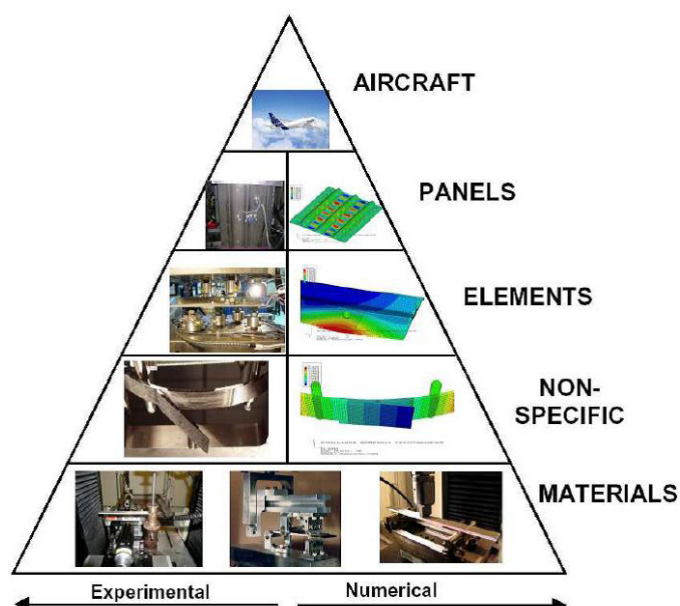
Fig. 1: Multi-level analysis applied to skin/stringer debonding (reproduced from ref [1]).
