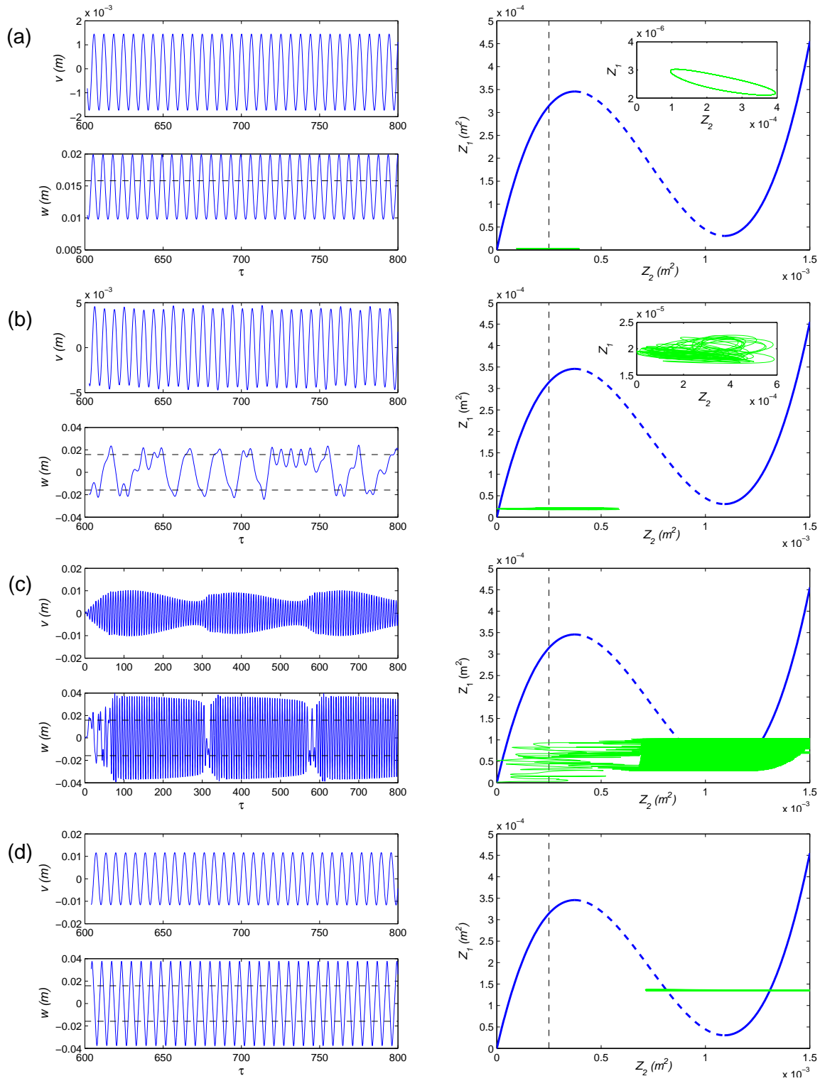
Fig. 5 Time-displacement response of LO and bistable NES, and the motion of the system projected into SIM (a) intra-well oscillation with G = 0.06 mm (b) chaotic inter-well oscillation with G = 0.1 mm (c) strongly modulated response with G = 0.42 mm (d) stable periodic response with G = 0.55 mm
