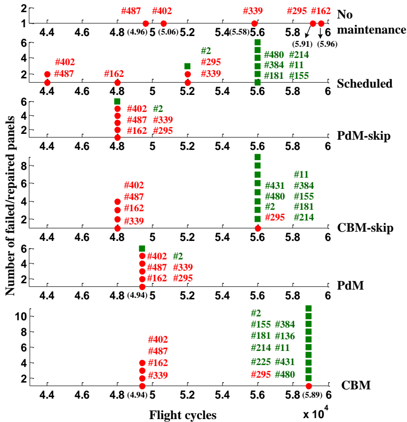
Figure 10. Different processes of aircraft #30
