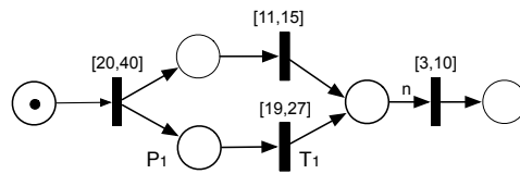
Figure 6. Time Petri Net Example
